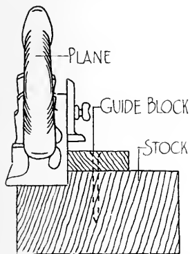
FIG. 67. GUIDE FOR RABBET PLANE.
